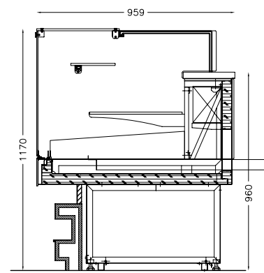
VETRINA PASTICCERIA CON CASSETTO MODELLO: GLAMOUR - EASY - FASHION PATISSERIE CABINET WITH DRAWER
