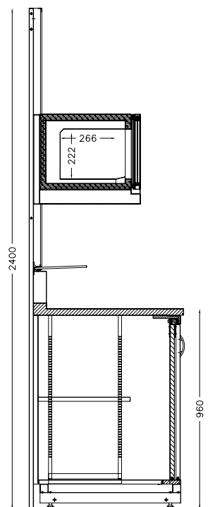
RETRO BANCO CON ALZATA REFRIGERATA MODELLO: GLAMOUR - EASY - FASHION BAR STATION WITH CHILLED STRUCTURE
