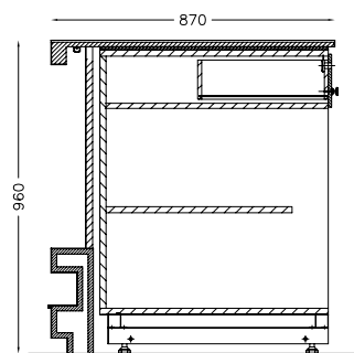
BANCO MULTIUSO H:96 MODELLO: EASY - FASHION MULTI-PURPOSE COUNTER H:96
