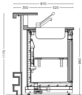
BANCO BAR MODELLO: GLAMOUR - EASY - FASHION BAR COUNTER
