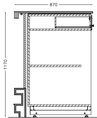
BANCO MULTIUSO H: 117 MODELLO: GLAMOUR - EASY - FASHION MULTI-PURPOSE COUNTER H:117
