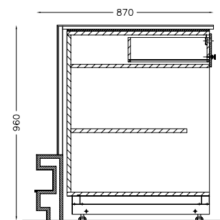
BANCO MULTIUSO H:96 MODELLO: GLAMOUR MULTI-PURPOSE COUNTER H:96
