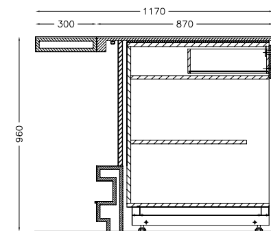
BANCO MULTIUSO H:96 OPTIONAL SCORRIVASSOIO MODELLO: EASY - FASHION MULTI-PURPOSE COUNTER H:96 OPTIONAL TRAY RAIL
