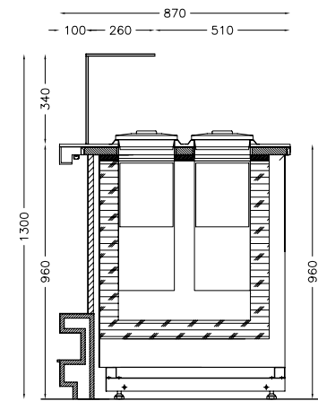
BANCO POZZETTO GELATO MODELLO: GLAMOUR - EASY - FASHION ICE CREAM WELL COUNTER
